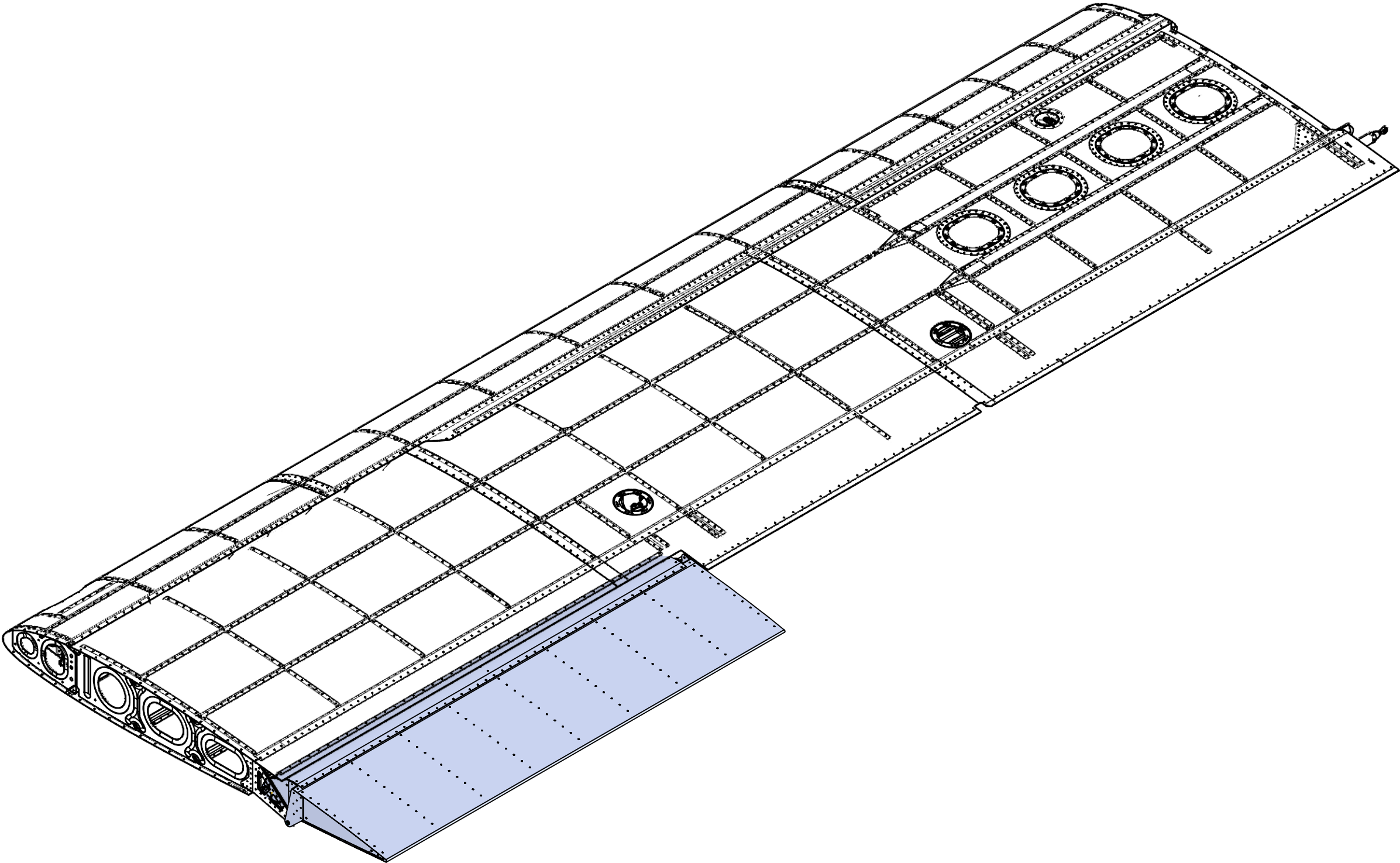
W-15512 AILERON ATTACH
