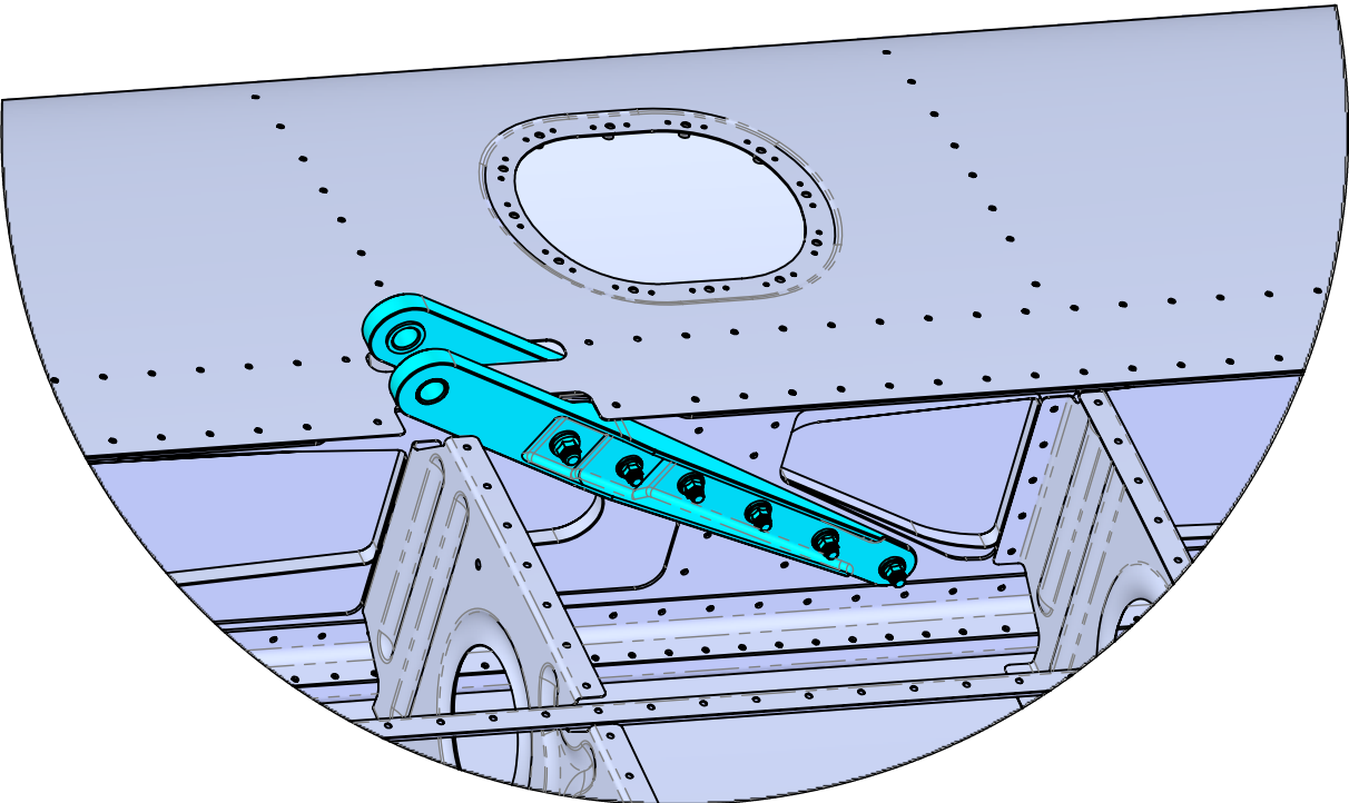
DETAIL A WING SKIN HIDDEN FOR CLARITY
