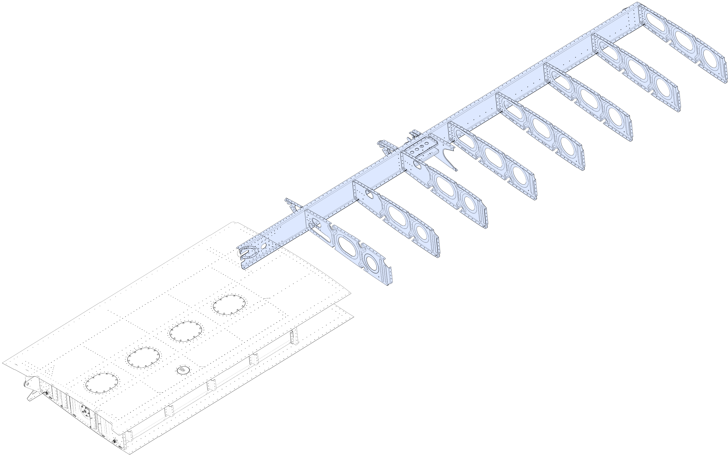
W-15505 REAR SPAR-TANK ASSEMBLY
